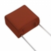
ECW-FA2J474J5 Panasonic Electronic Components CAP FILM 0.47UF 5% 630VDC RADIAL
