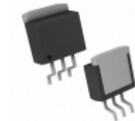
MCP1826S-3002E/EB Microchip Technology IC REG LDO 3V 1A 3DDPAK
