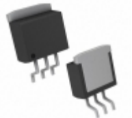
MCP1826S-3302E/EB Microchip Technology IC REG LDO 3.3V 1A 3DDPAK
