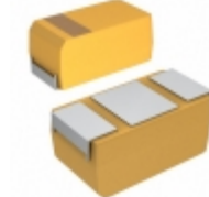
CWR09MC685KP KEMET CAP TANT 6.8UF 10% 35V 2915
