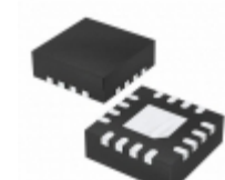
ISL43640IRZ-T Intersil IC MUX/DEMUX 4X1 16QFN
