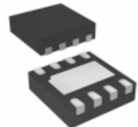
AP7361-12FGE-7 Diodes Incorporated IC REG LDO 1.2V 1A DFN-3030-8
