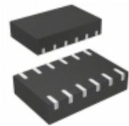
STM6600CS25DM6F STMicroelectronics IC SUPERVISOR 3.4V 12TDFN
