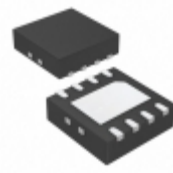
LTC4068EDD-4.2#PBF ADI (Analog Devices, Inc.) IC CHARGER BATT LI-ON 8-DFN
