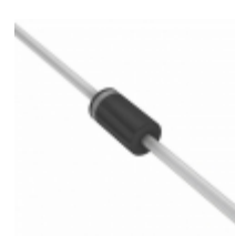
BZW04-48B R0G TSC (Taiwan Semiconductor) TVS DIODE 47.8V 77V DO204AL
