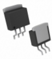
MIC39150-2.5WU-TR Microchip Technology IC REG LDO 2.5V 1.5A TO263-3
