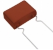
ECW-F2334HAB Panasonic Electronic Components CAP FILM 0.33UF 3% 250VDC RADIAL
