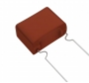
ECW-F2275HAB Panasonic Electronic Components CAP FILM 2.7UF 3% 250VDC RADIAL
