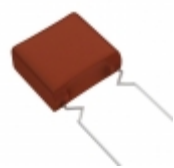
ECW-F2275JAQ Panasonic Electronic Components CAP FILM 2.7UF 5% 250VDC RADIAL
