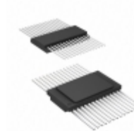
AT28C256-20FM/883 Microchip Technology IC EEPROM 256KBIT 200NS 28FLATPK
