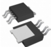
BAJ0BC0WFP-E2 Rohm Semiconductor IC REG LDO 10V 1A TO252-5
