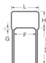
ECQ-P1H273GZ3 Panasonic Electronic Components CAP FILM 0.027UF 2% 50VDC RADIAL
