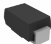
BZG05C62-E3-TR3 Vishay / Semiconductor - Diodes Division DIODE ZENER 62V 1.25W DO214AC
