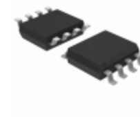
MIC29201-3.3BM Microchip Technology IC REG LDO 3.3V 0.4A 8SOIC
