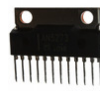
AN5273 Panasonic Electronic Components IC AUDIO AMP 2CH 4W SIL-12 W/FIN
