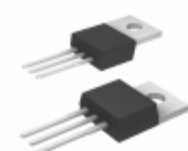
TIP127G ON Semiconductor TRANS PNP DARL 100V 5A TO220AB
