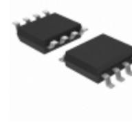
BR93L86RF-WE2 Rohm Semiconductor IC EEPROM 16KBIT 2MHZ 8SOP
