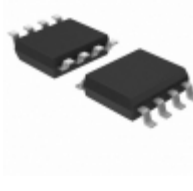
BR93L86RFJ-WE2 Rohm Semiconductor IC EEPROM 16KBIT 2MHZ 8SOP-J
