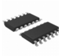
AD8040ARZ Analog Devices Inc. IC OPAMP GP 125MHZ RRO 14SOIC
