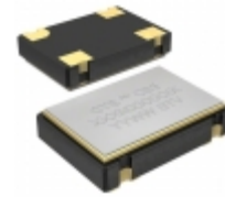
CB3LV-2I-83M3300 CTS-Frequency Controls OSC XO 83.33MHZ HCMOS TTL SMD
