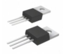
D44H8 ON Semiconductor TRANS NPN 60V 10A TO220AB
