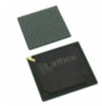
LFE3-95E-8FN1156I Lattice Semiconductor Corporation IC FPGA 490 I/O 1156FBGA
