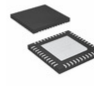
PIC18LF47K42-E/ML Micrel / Microchip Technology IC MCU 8BIT 128KB FLASH 44QFN
