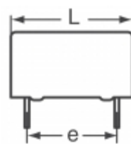
B32794D4355K EPCOS (TDK) CAP FILM 3.5UF 10% 1.05KVDC RAD
