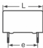
B32794D4155K EPCOS (TDK) CAP FILM 1.5UF 10% 1.05KVDC RAD
