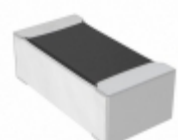
PCF0603R-931RBT1 TT Electronics/Welwyn RES SMD 931 OHM 0.1% 1/16W 0603
