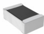
PCF0805-12-100KBT1 TT Electronics RES SMD 100K OHM 0.1% 1/10W 0805
