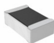
PCF0805-12-150KBT1 TT Electronics/Welwyn RES SMD 150K OHM 0.1% 1/10W 0805
