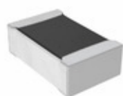
PCF0805-12-150KBT1 TT Electronics RES SMD 150K OHM 0.1% 1/10W 0805
