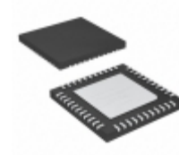
PIC24F16KM204-E/ML Microchip Technology IC MCU 16BIT 16KB FLASH 44QFN
