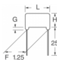
ECQ-P6393JU Panasonic Electronic Components CAP FILM 0.039UF 5% 630VDC RAD
