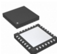
PIC16F18856-I/ML Microchip Technology IC MCU 8BIT 28KB FLASH 28QFN
