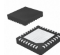
PIC16F18856-I/MV Microchip Technology IC MCU 8BIT 28KB FLASH 28UQFN
