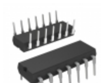
MCP4251-503E/P Microchip Technology IC DGTL POT 50K 2CH 14DIP
