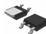
MURD340T4G ON Semiconductor DIODE GEN PURP 400V 3A DPAK
