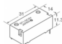
ST2-DC9V Panasonic Electric Works RELAY GENERAL PURPOSE DPST 8A 9V
