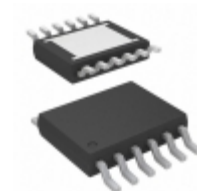
LTC4419CMSE#PBF ADI (Analog Devices, Inc.) IC SOURCE SELECTOR SWITCH 12MSOP
