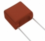
ECW-F2475HA Panasonic Electronic Components CAP FILM 4.7UF 3% 250VDC RADIAL
