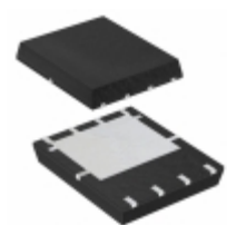
RS1G260MNTB Rohm Semiconductor MOSFET N-CH 40V 26A 8HSOP
