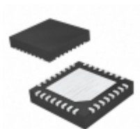
PIC24EP64GP202T-I/MM Microchip Technology IC MCU 16BIT 64KB FLASH 28QFN
