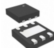
MIC5393-SGYMX-T5 Microchip Technology IC REG LDO 3.3V/1.8V 0.15A 6TDFN
