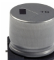
EEV-TG2A221M Panasonic Electronic Components CAP ALUM 220UF 20% 100V SMD
