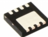
FDMC86139P Fairchild/ON Semiconductor MOSFET P-CH 100V 4.4A 8MLP
