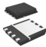
FDMC86160ET100 Fairchild/ON Semiconductor MOSFET N-CH 100V 9A POWER33
