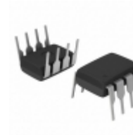
CT474 Coto Technology RELAY SSR SPST-NC 400V 90MA 8DIP
