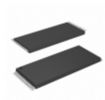
AT29C020-12TI Microchip Technology IC FLASH 2MBIT 120NS 32TSOP
