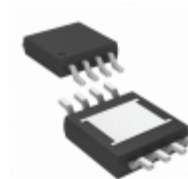
LT5400AIMS8E-1#TRPBF Linear Technology RES ARRAY 4 RES 10K OHM 8TSSOP
