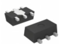
S-1135C25-U5T1G SII Semiconductor Corporation IC REG LINEAR 2.5V 0.3A SOT89-5
