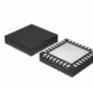
HMC742HFLP5E Analog Devices Inc. IC AMP DVGA 6-BIT 0.5DB 32-QFN
