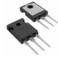
IRGPC50U Infineon Technologies IGBT UFAST 600V 55A TO-247AC
