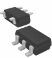
MCP40D19T-103E/LT Microchip Technology IC DGTL POT 10K 128TAPS SC70-5
