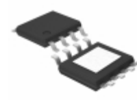
BD15IA5MEFJ-ME2 Rohm Semiconductor IC REG LDO 1.5V 0.5A 8HTSOP
