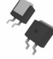
IXTA10P50P IXYS MOSFET P-CH 500V 10A TO-263
