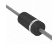
P6KE8.2-E3/73 Vishay Semiconductor Diodes Division TVS DIODE 6.63VWM 12.5VC DO204AC
