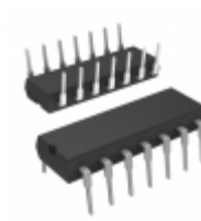
AD8044ANZ Analog Devices Inc. IC OPAMP VFB 160MHZ RRO 14DIP
