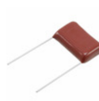
ECQ-E6474KF Panasonic Electronic Components CAP FILM 0.47UF 10% 630VDC RAD
